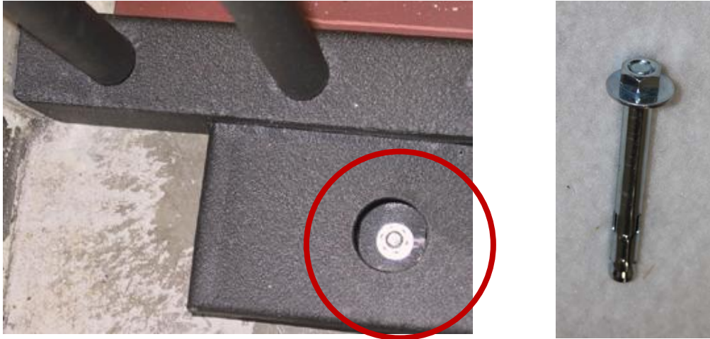
Picture 8-8 Rail anchored to floor with 3" x 3/8" anchor bolt
